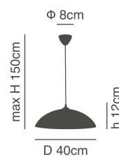
77-8221-28 SE21-WH-40 1xE27, max 60W, 230V
